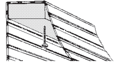
2” or 3” Screw
